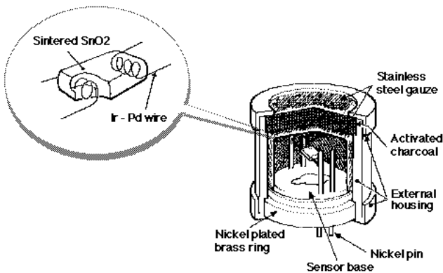
Figure 1 - Sensor structure
